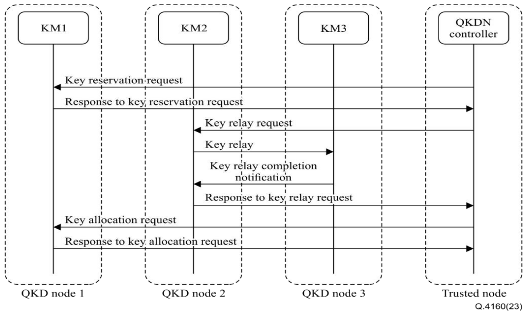
Figure: 10B Typical signalling procedures for key relay for a centralized QKDN with key reservation
