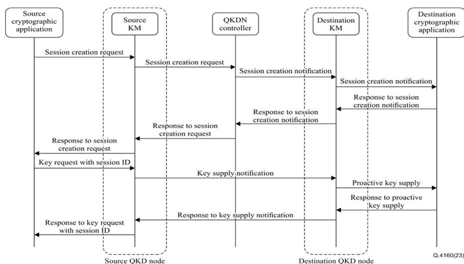
Figure 9 Typical signalling procedures for proactive key supply mode implemented by two QKD nodes
