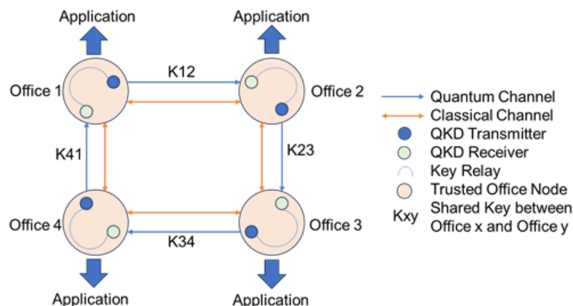
Figure 3C: QKD Ring network topology
