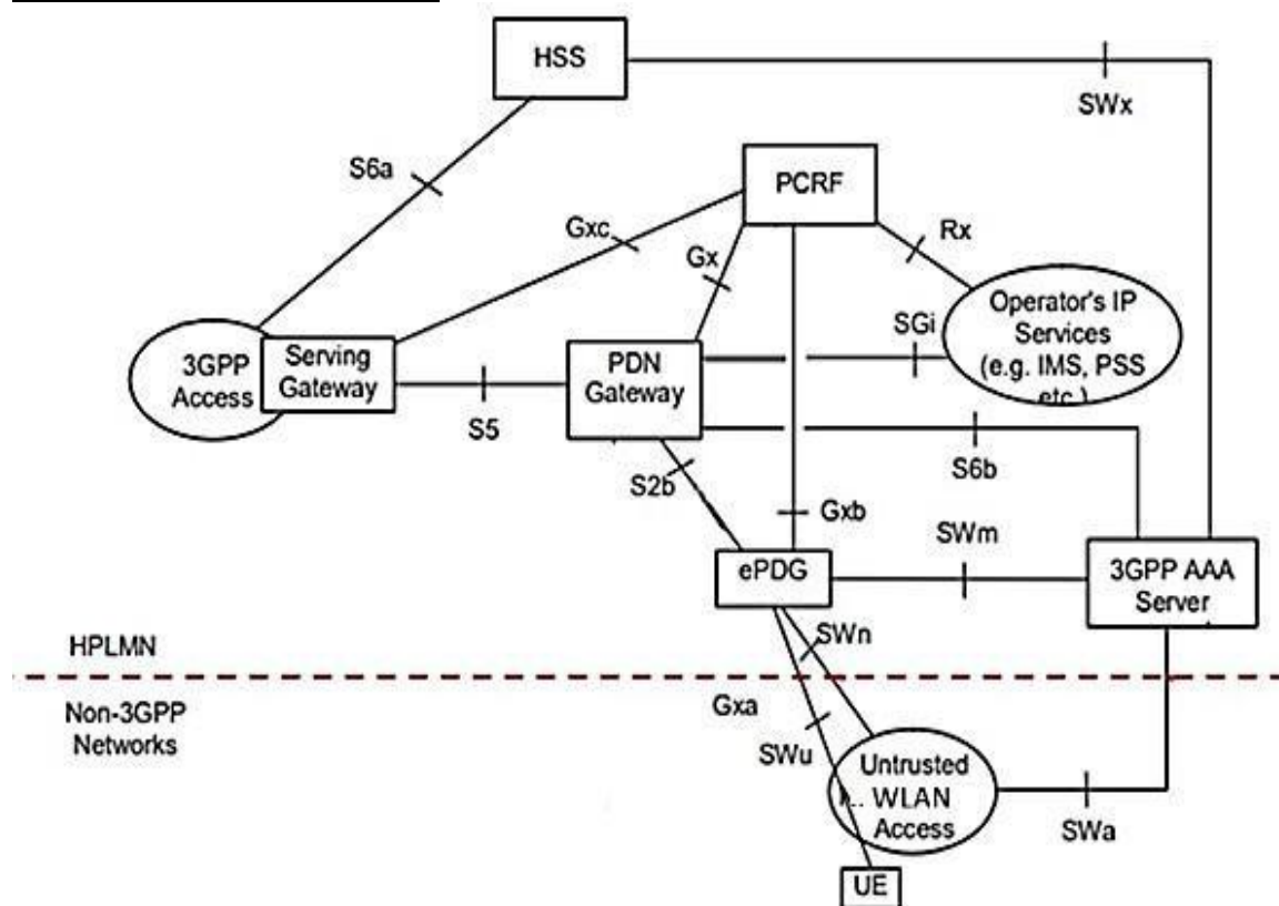
Figure 2: Functional Architecture for Untrusted WLAN Access to EPC 3
