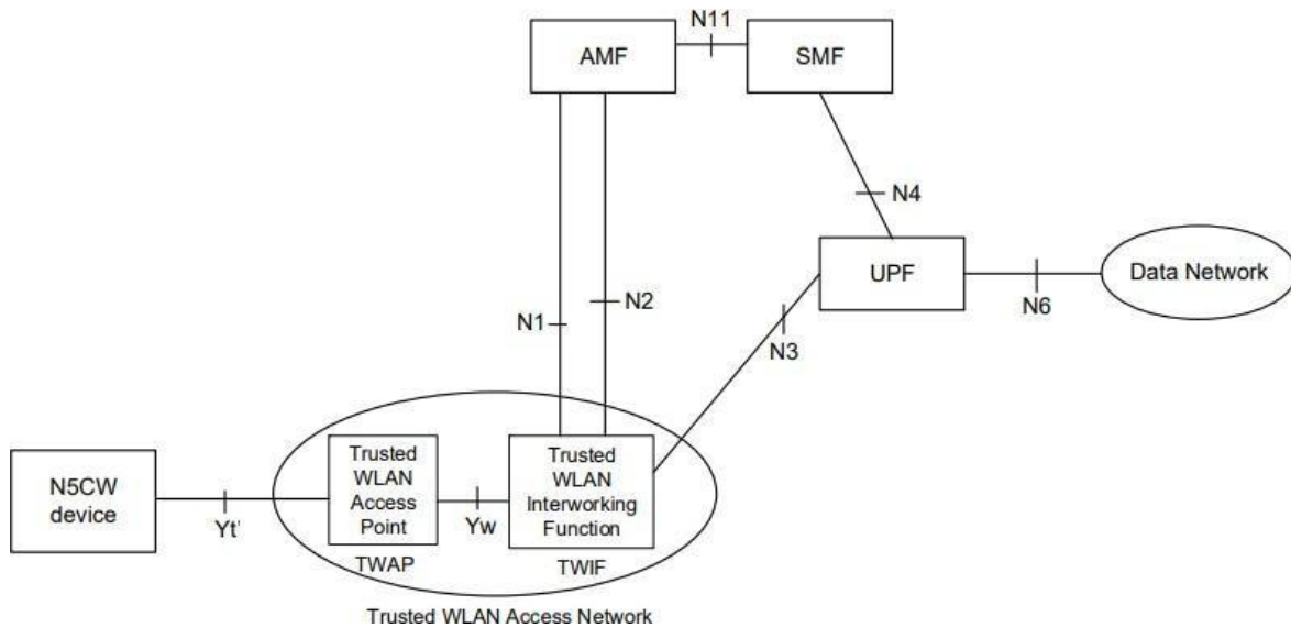
Figure 5: Functional architecture of 5GC interworking with TWAN for N5CW devices 6 The key network elements involved in interworking between the TWAN and the 5GC through the TWIF are as follows:
