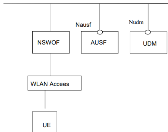
Figure 6 (b). Service based reference architecture to support authentication for NSWOF in 5GS 8
