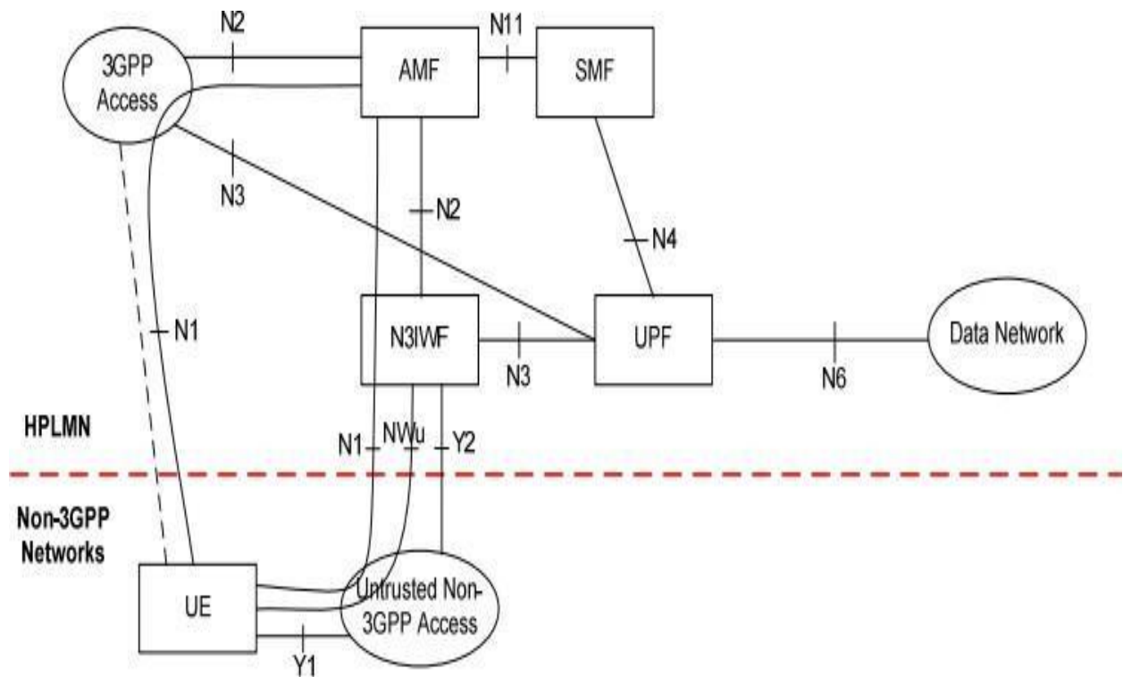
Figure 3: Functional architecture of 5G core network interworking with untrusted Non- 3GPP Access 4
