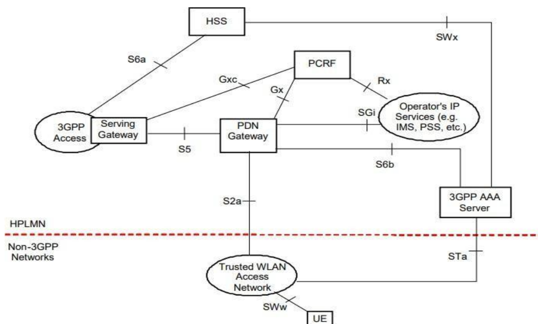
Figure 1: Functional Architecture for Trusted WLAN Access to EPC 2
