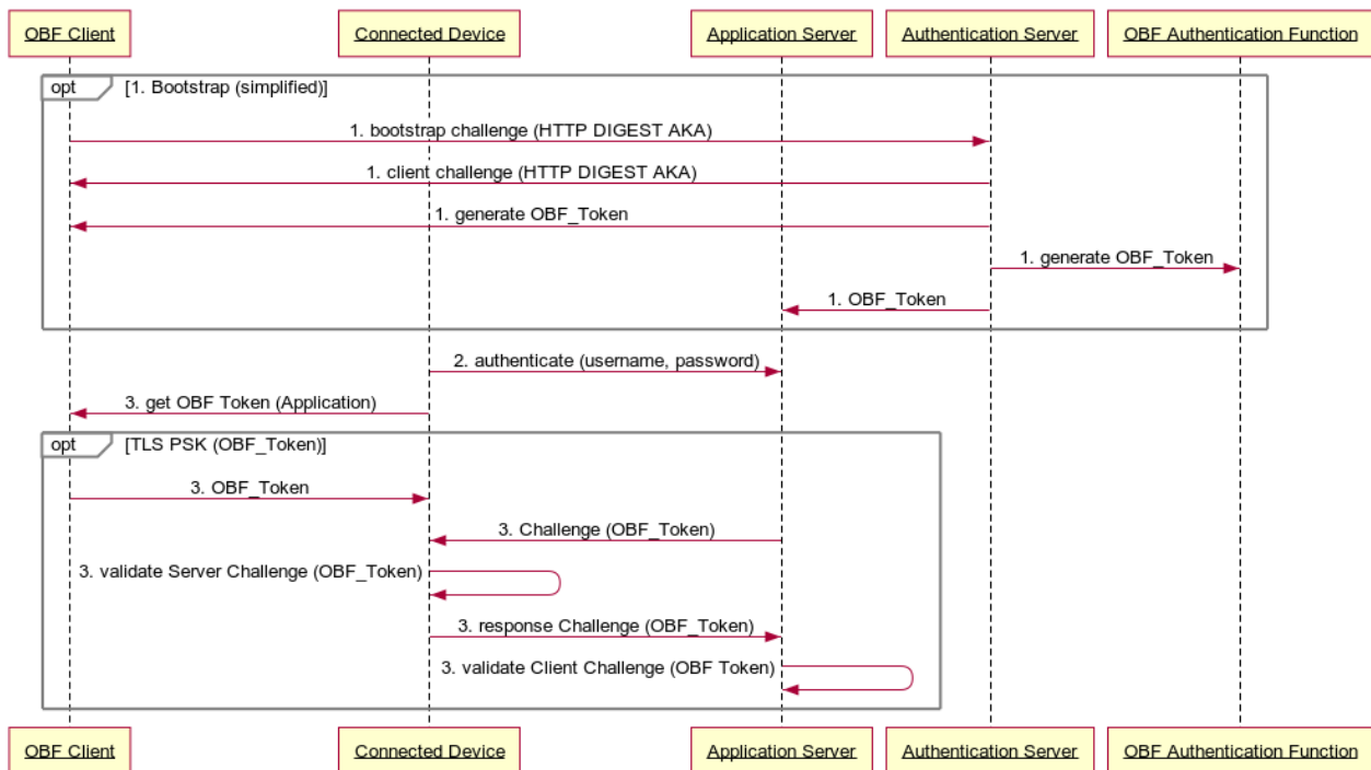
Figure 5: Authentication Sequence Diagram
