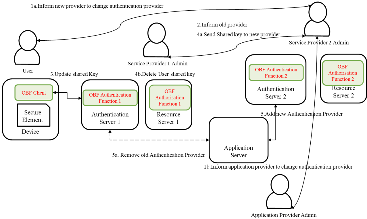
Figure 5: Authentication Provider Switch (Asymmetric keys)
