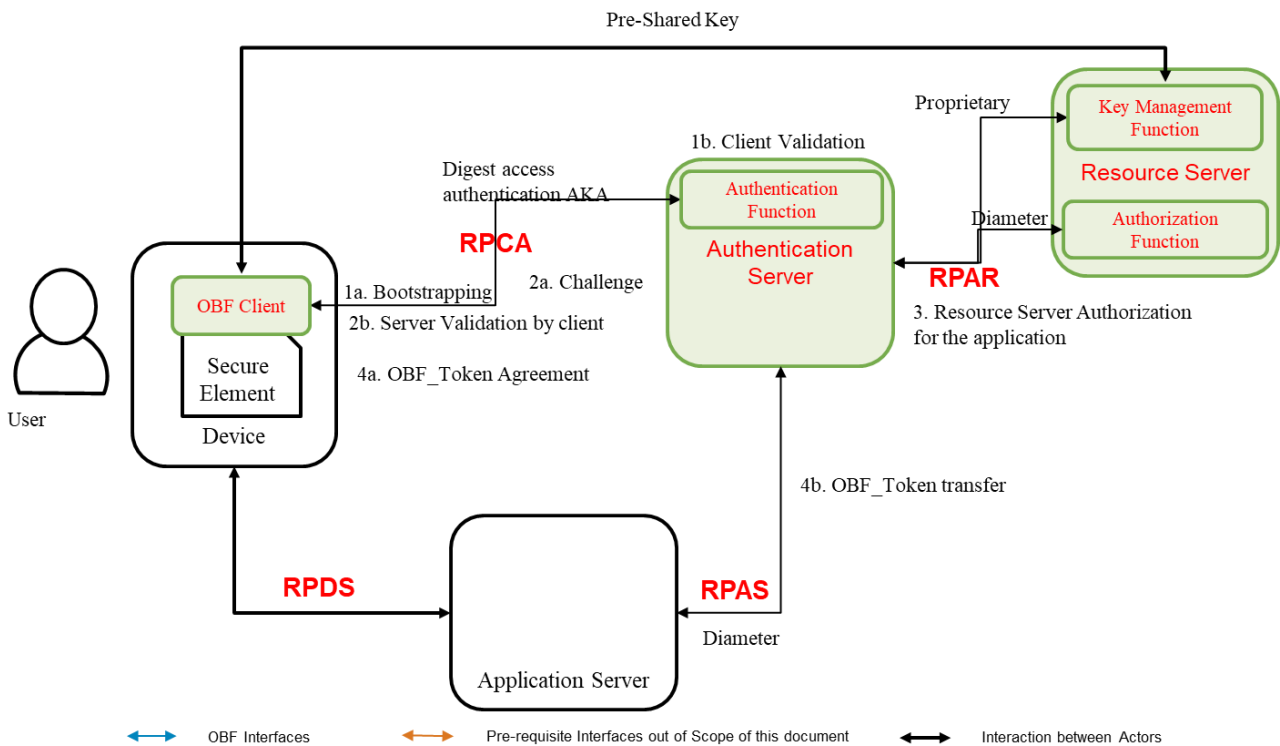
Figure 6: Bootstrapping and Session Key Management
